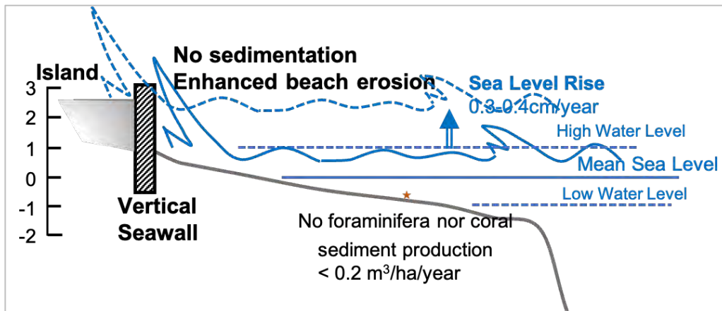
Fig.6. Loss of natural land-building processes caused by vertical seawalls and coral reef degradation.
