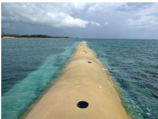
Fig. 19. Sand tube (left, Geotube Marine) and permeable sand trap deployed on Barasu Island, Iriomote-jima.
