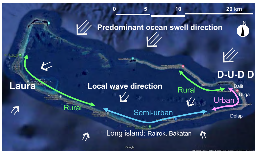
Fig. 11. Spatial features of Majuro Atoll, showing community types and predominant wave conditions.
