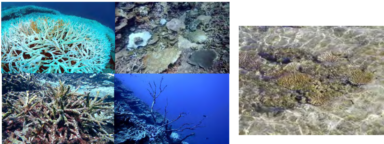
Fig. 7. Coral reef degradation inside and outside Majuro Atoll.
