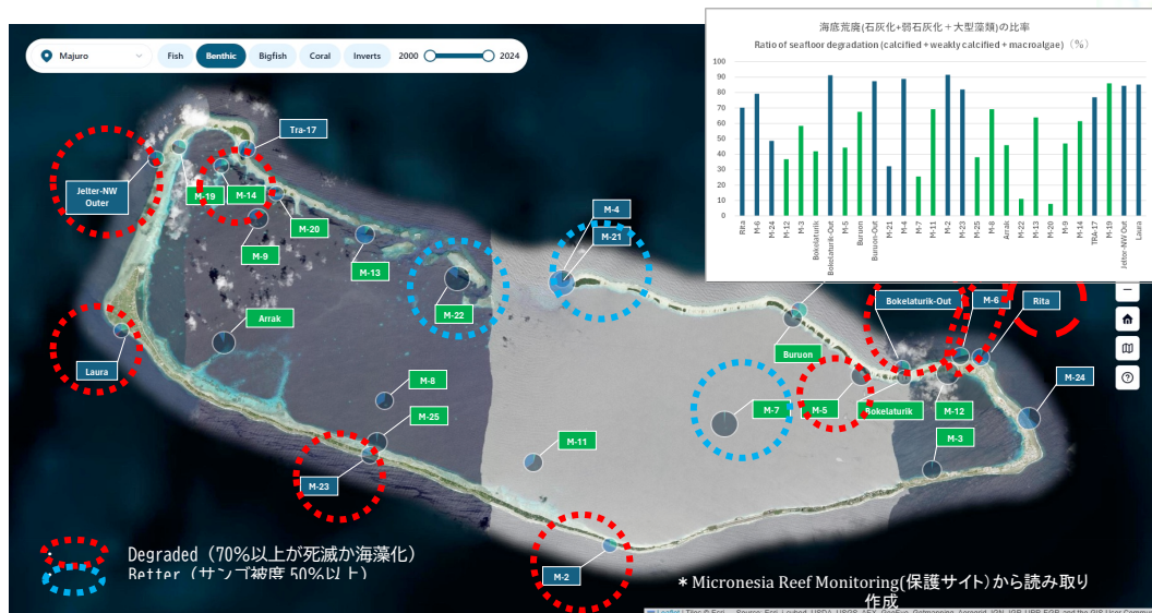
Fig. 8. Results of the coral reef environmental survey in Majuro Atoll (Created from Micronesia Reef Monitoring, University of Guam)
