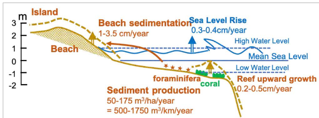
Fig. 5. Healthy coral reefs create and sustain atoll land under sea-level rise.
