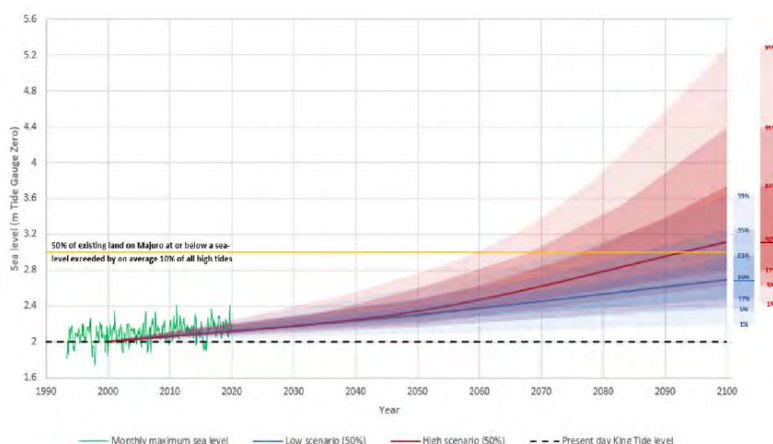
Fig. 4. Sea level observations and projections for Majuro (Barber et al., 2019).
