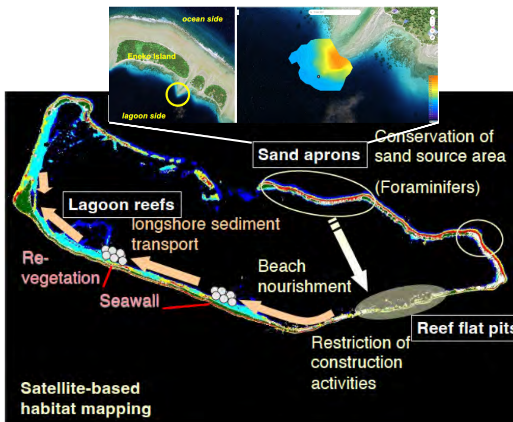
Fig. 20. Concept of beach nourishment using lagoon-floor sediments and sand aprons formed around the northern islets.
