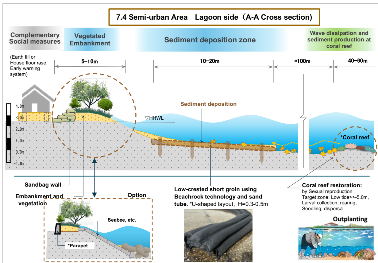
Fig. 28. Conceptual cross-section of Semi-urban Areas – Lagoon Side.
