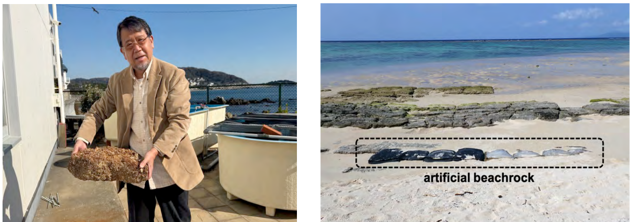
Fig. 21. Coral sand/gravel that solidified within two weeks (left) and artificial beachrock on a shore (right).
