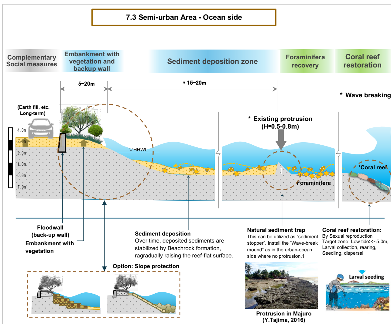
Fig. 26. Conceptual cross-section of Semi-urban Areas – Ocean Side.
