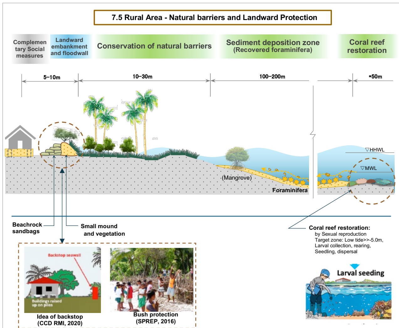
Fig. 30. Conceptual cross-section of Rural Areas – Ocean and Lagoon Sides.
