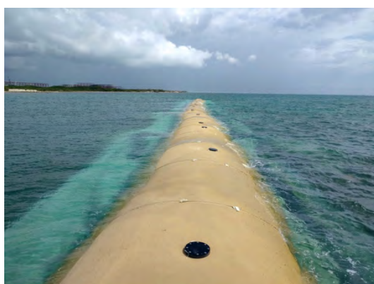
Fig. 19. Sand tube (left, Geotube Marine) and permeable sand trap deployed on Barasu Island, Iriomote-jima.
