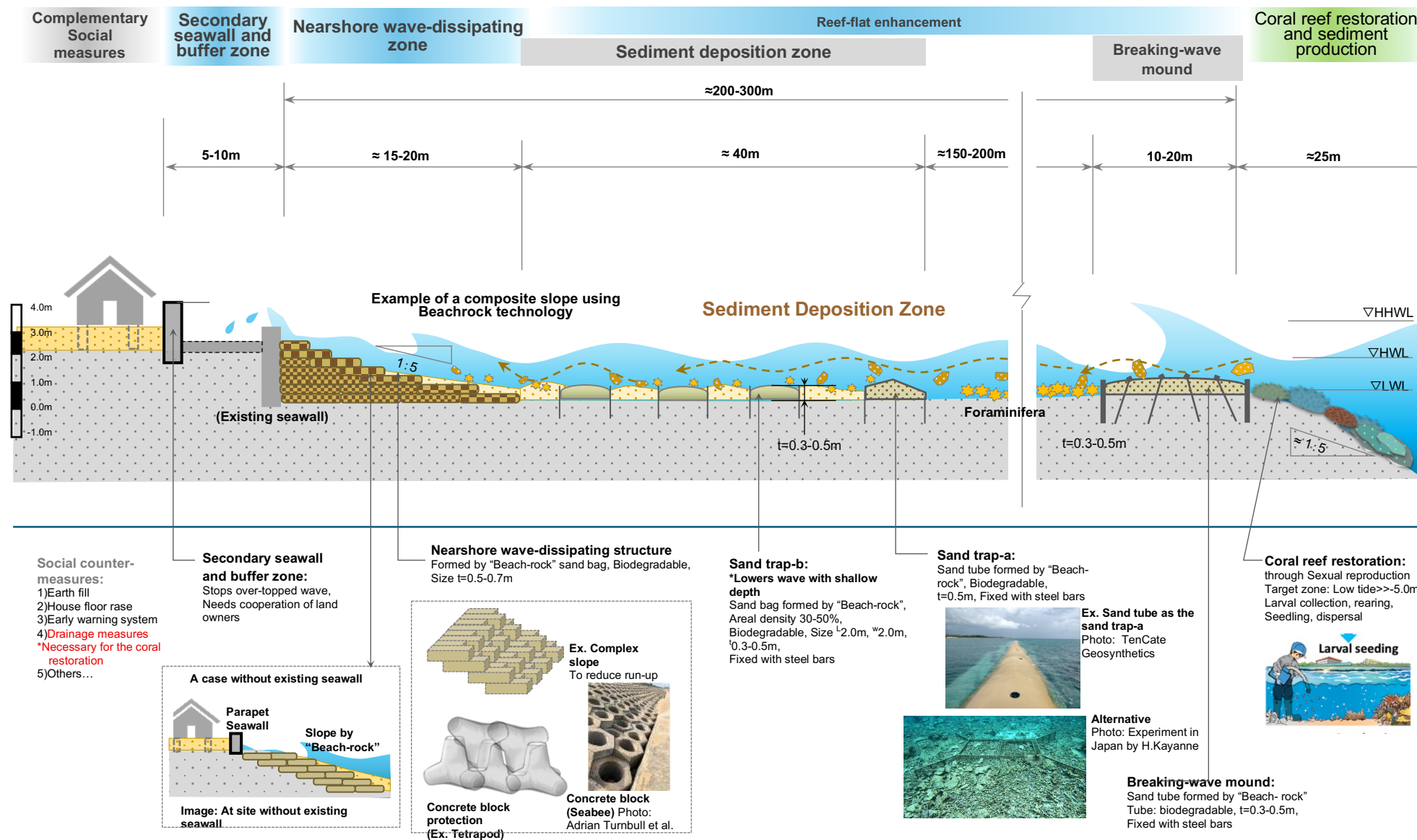
Fig. 23. Conceptual cross-section of Urban Areas – Ocean Side
