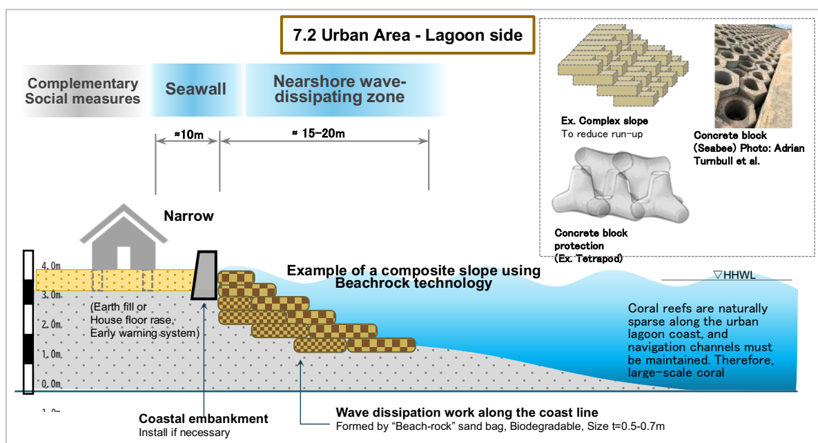
Fig. 25. Conceptual cross-section of Urban Areas – Lagoon Side.
