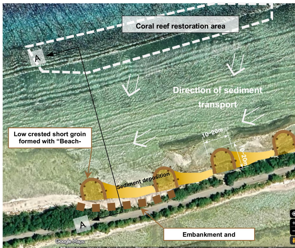
Fig. 29. Plane diagram of semi-urban lagoon coast.
